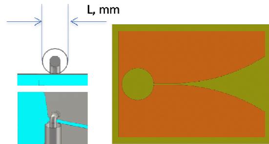
Fig.1. Antenna's geometry
