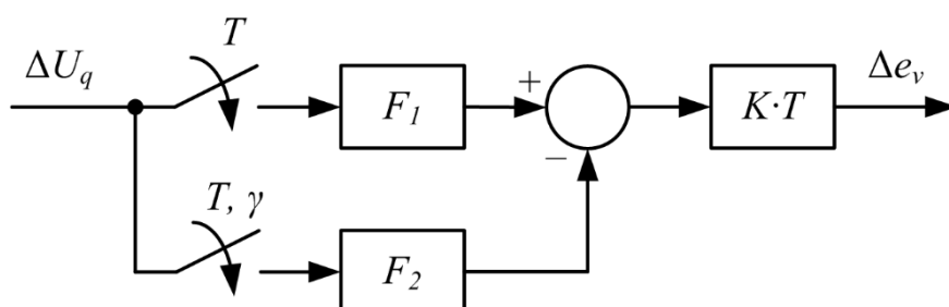
Fig. 5. Pulse model of a pulse-width modulated converter with a two-sided reference signal
