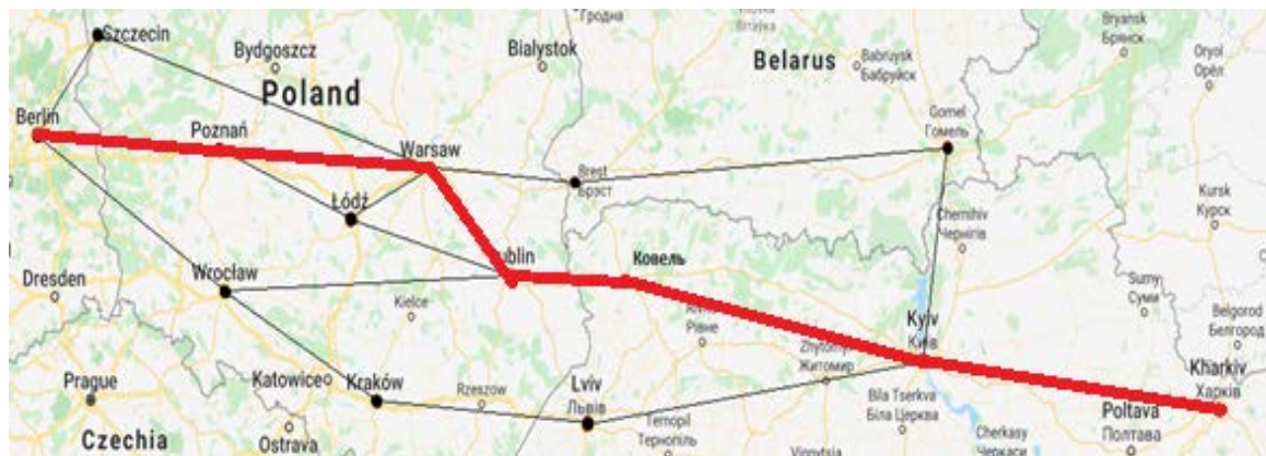
Fig. 2. Transport Route Using the GA Method
