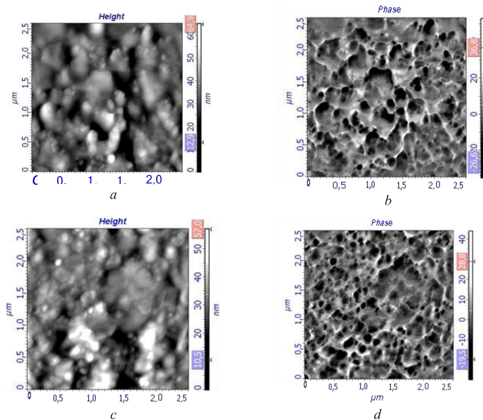
Fig.1. AFM image of chips from samples with ZrO 2 –30 wt. % Al 2 O 3 composition sintered at 1,200 °C: a – fracture height in samples prepared from P–2 powder; b – structure of fracture in samples prepared from P–2 powder; c – fracture height in samples prepared from P–3 powder; d – structure of fracture in samples prepared from P–3 powder
